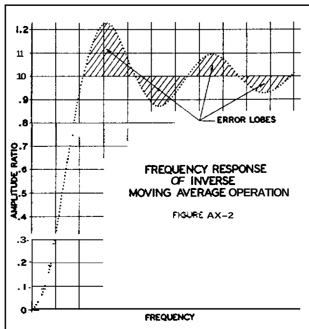
HOW An Inverse Moving Average Works
